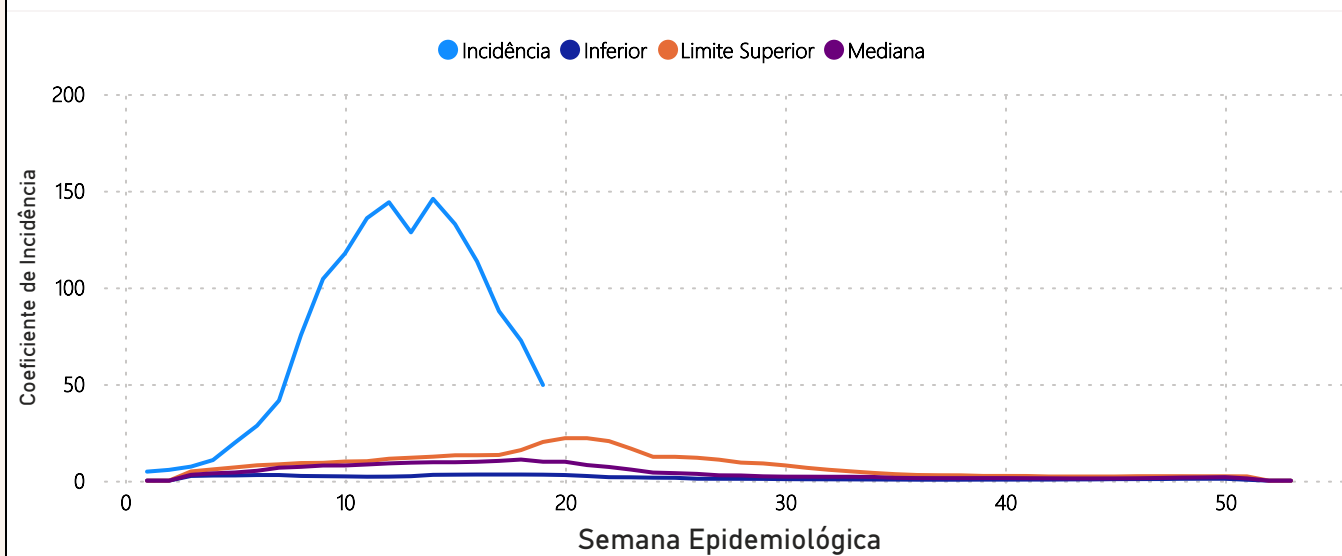
Diagrama de Controle Dengue, Bahia, 2024
